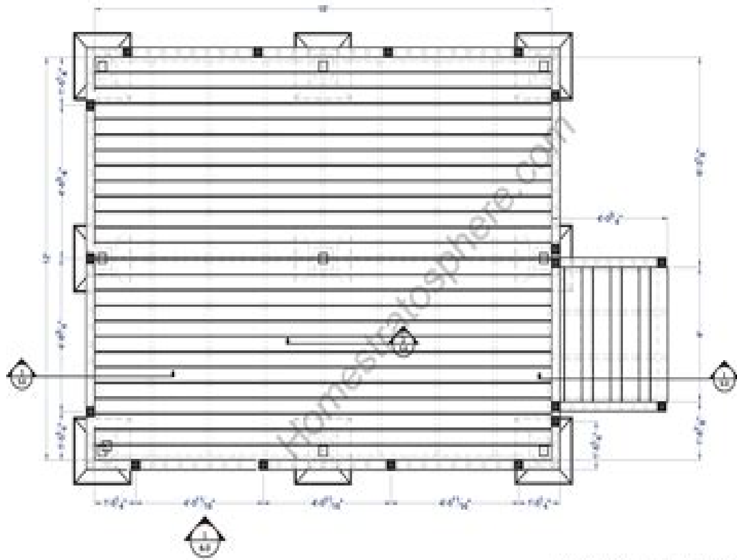
1 TOP VIEW DECK 12'X16' Scale 1/8" = 1'
