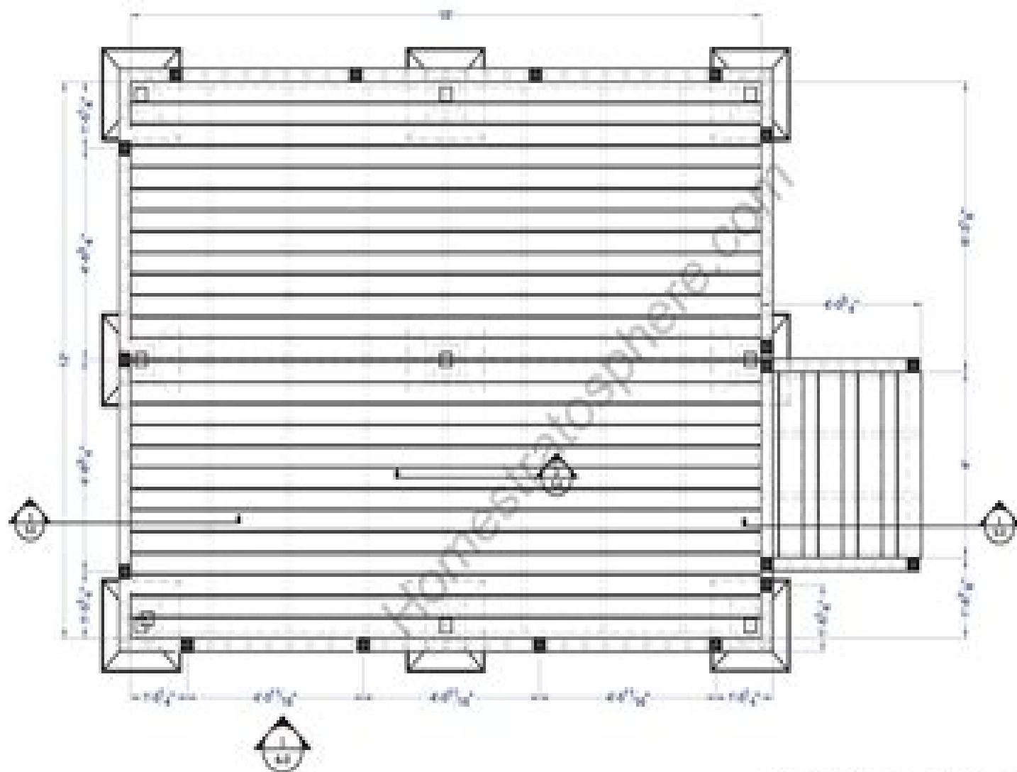
1 TOP VIEW DECK 12'X16'
